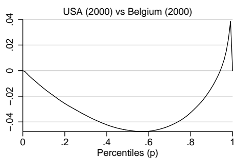
Figure 2: Difference between Lorenz curves
