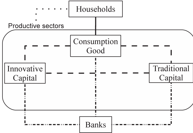
Figure 1: Flow diagram of the model: Households consume (solid line) all their wages (dotted line). All productive sectors use capital goods to produce (dashed line). They invest and pay their wage bills using bank loans (dash-dotted line).
