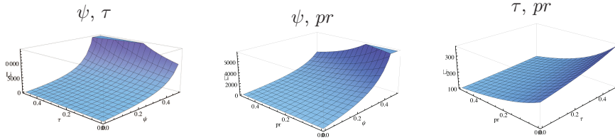
Figure 2: Credit needed to finance innovation ( L_i ) changes when the targeted market share \psi , the targeted growth rate \tau and the productivity gain pr vary. The higher the market share and the growth rate, the higher L_i . The higher the productivity gain, the lower L_i .
