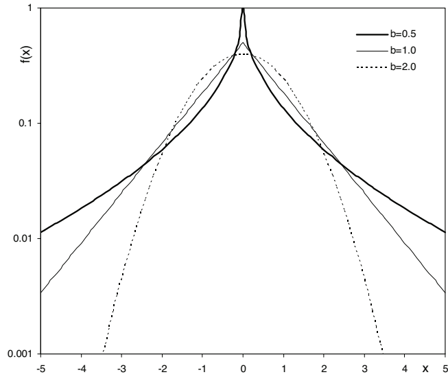
Figure 1: The exponential-power (EP) density for m = 0, a = 1 and different shape-parameter values: (i) b = 2 : Gaussian density; (ii) b = 1 : Laplace density; (iii) b = 0.5 : EP with super-Laplace tails. Note: Log scale on the y-axis
