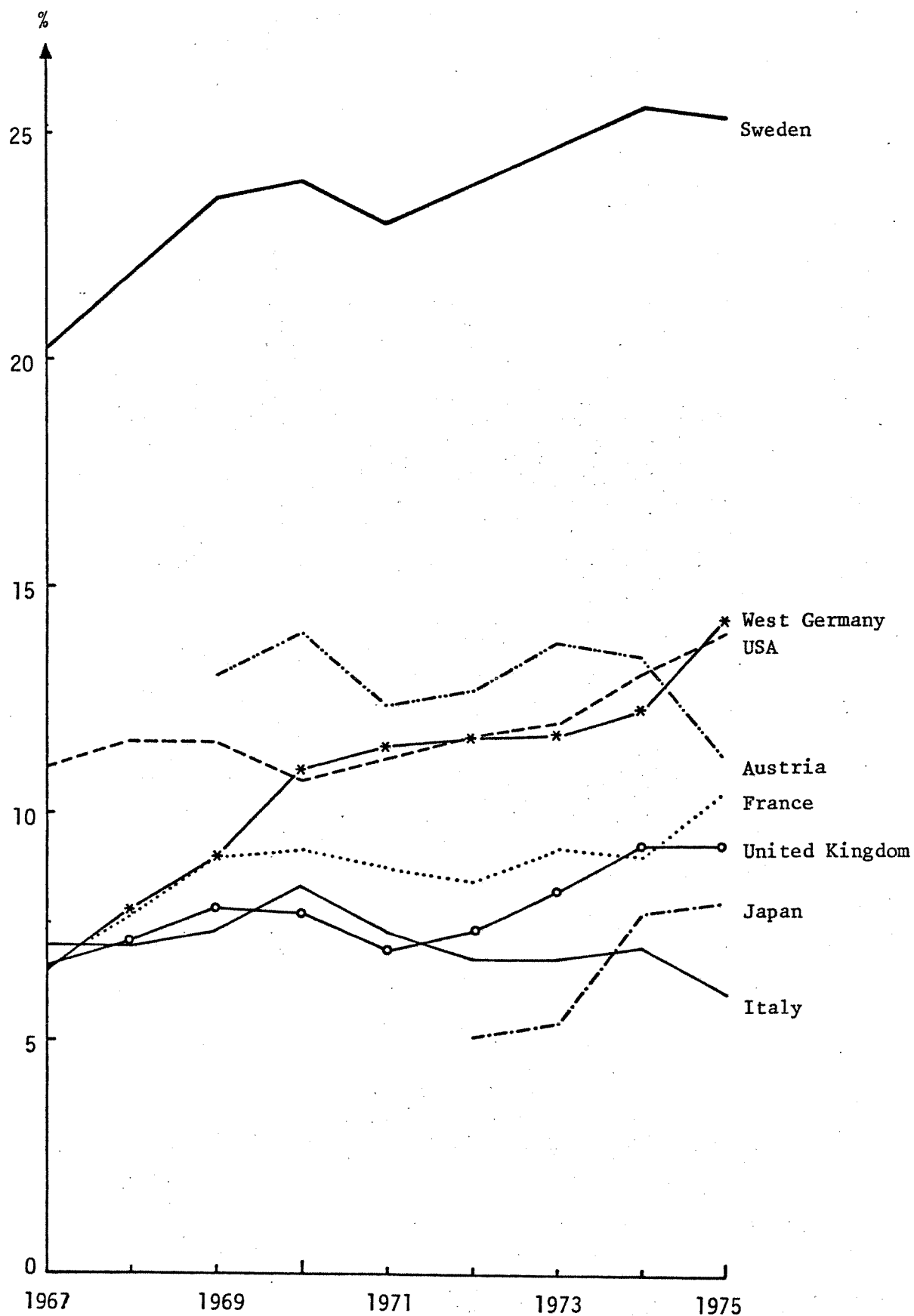
Figure 5. The share of alloyed steel in total crude steel production in certain countries 1967-1975 Percent.
