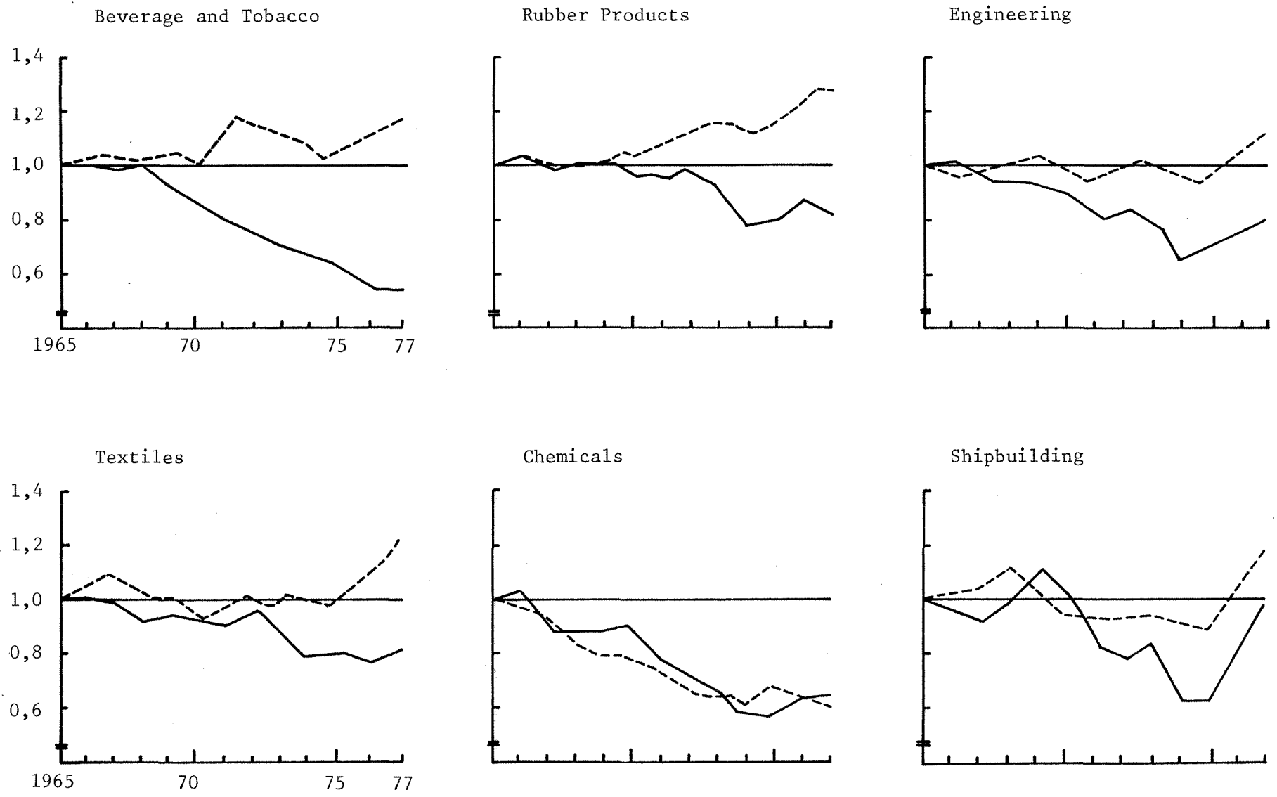
Figure 4B Specific use of electricity and oil in manufacturing sectors, 1965-1977. (1965 = 1). Electricity (- - -). Oil (-----)
