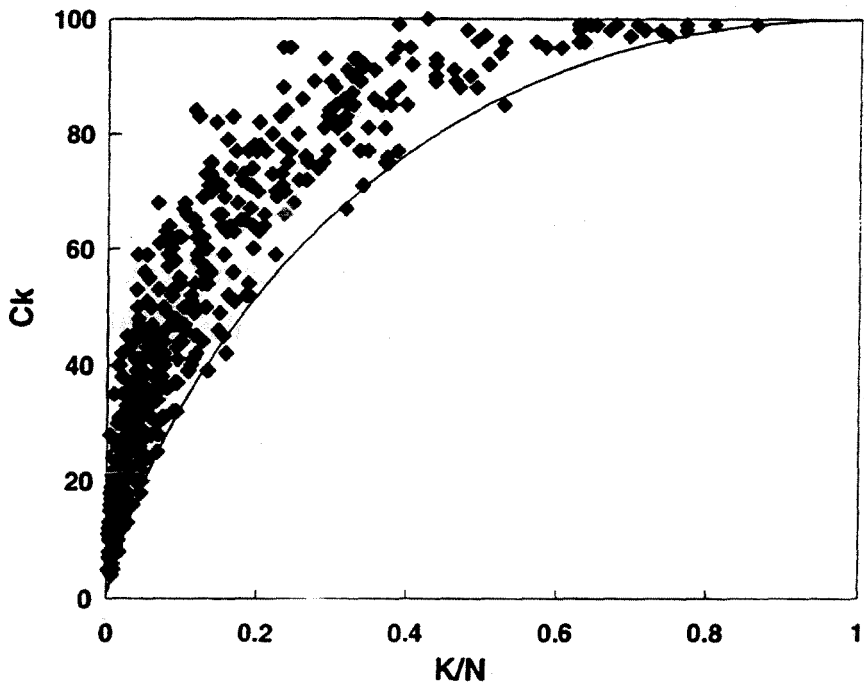
Figure 5. Testing Proposition 1. The top panel shows the scatter diagram of C_k against k/N for pooled data ( k = 4, 8 and 20 ) for the U.S., 1987, at the 4-digit level. The Lorenz curve is the limiting curve defined by Proposition 1 (equation (11)'). The bottom panel shows data for Germany, 1990 ( k = 3, 6, 10 and 25 ).
