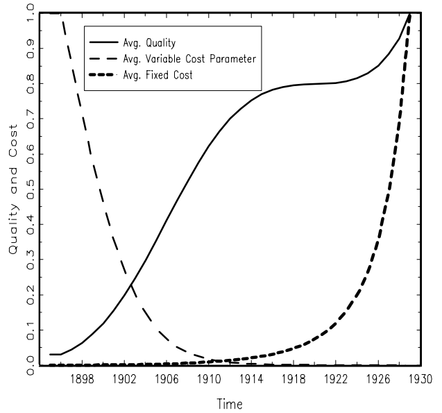
Fig. 9. Investment in Quality and Cost Improvements
