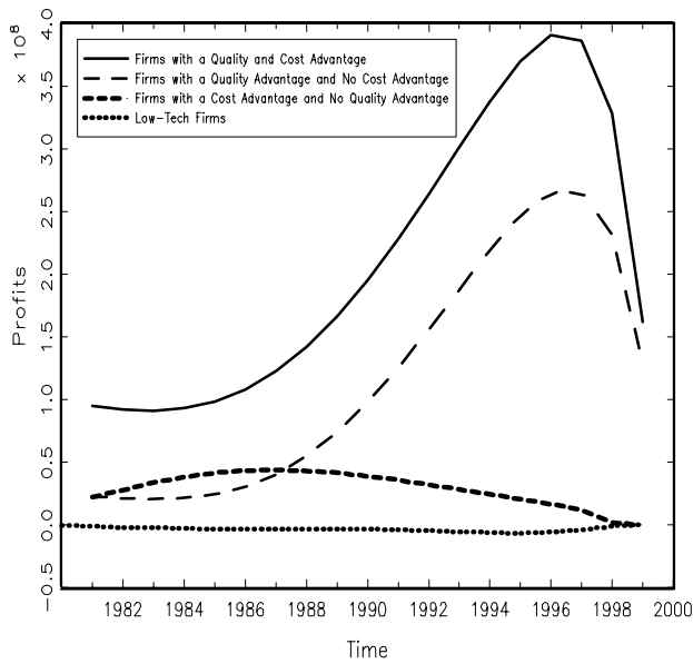
Fig. 16. Profits of the Various Types of Firms
