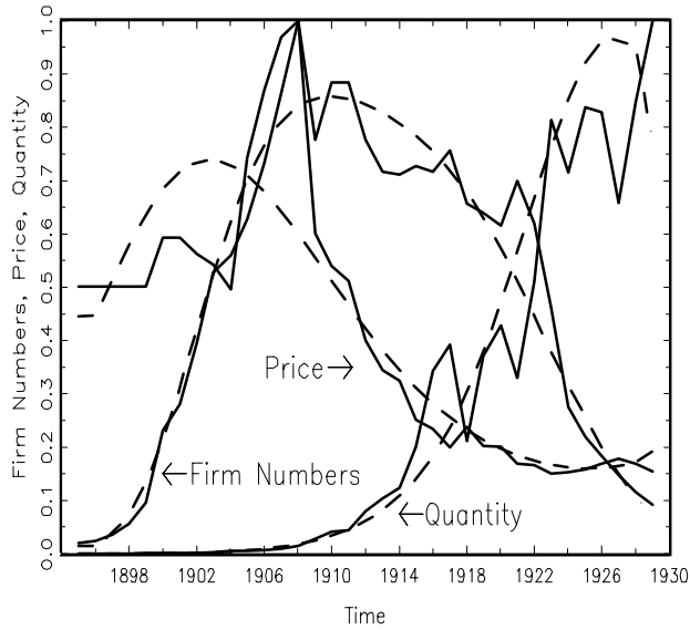
Fig. 6. Firm Numbers, Price, and Market Quantity (Solid lines: data Dashed lines: simulation results)
