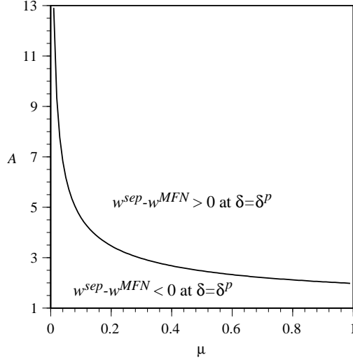
Figure 5: Zero contour of w^{\text{sep}} - w^{\text{MFN}} .
