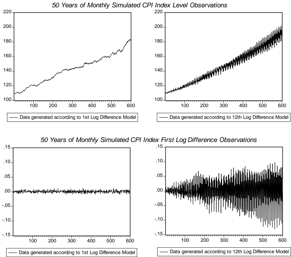
Figure 1: Simulated CPI Levels and 1st Log Differences Simulation Models Calibrated Using Monthly U.S. Data
