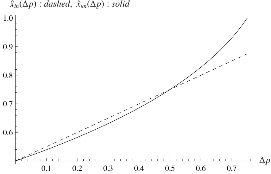
Location of the indifferent informed and uninformed consumer (= demand of firm A) as a function of \Delta p for parameter values of t = 1 and \lambda = 3 ; \Delta \bar{p} = 0.8348 , \Delta \bar{p} = 3/4 and \Delta \hat{p} = 0.2789 .
