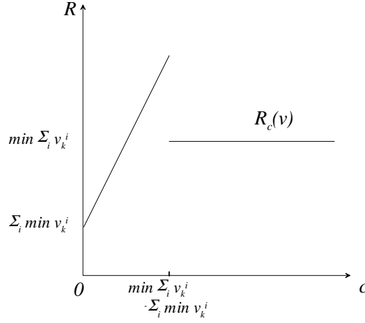
Figure 1: Realized Revenue R_c(v) as a function of c (fixing v such that bundling is inefficient).
