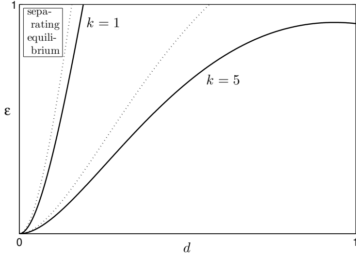
Figure 1: Existence of a separating equilibrium for the uniform-price auction under Cournot competition with uniformly distributed costs.
