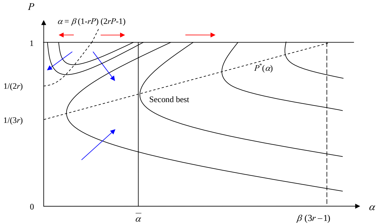
Figure 1 – Social welfare contours in (\alpha, P) -space
