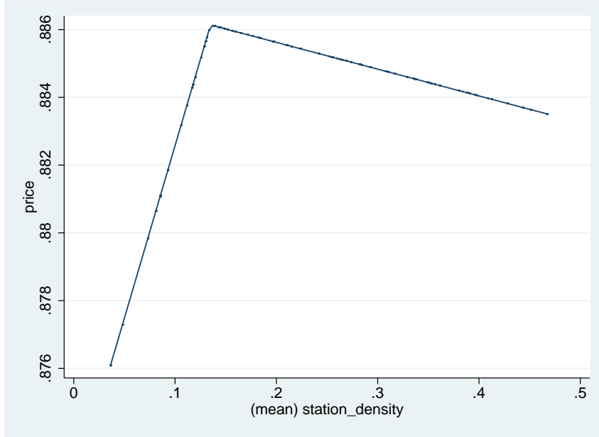
Figure 6: Predicted prices
