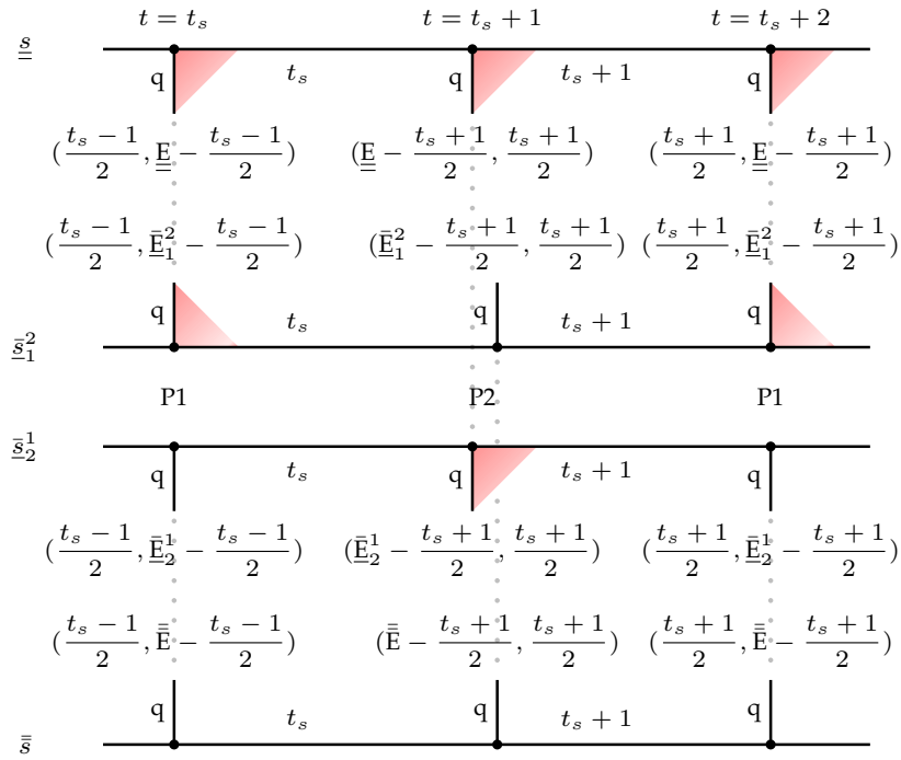
Figure 2: The end of the equilibrium 'preplay'-phase at t_s for odd \lfloor \bar{E} \rfloor .
