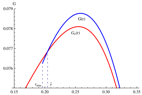
Figure 2: Uniform distribution
