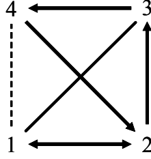
Figure 1: Graphical representation of a network of relations
