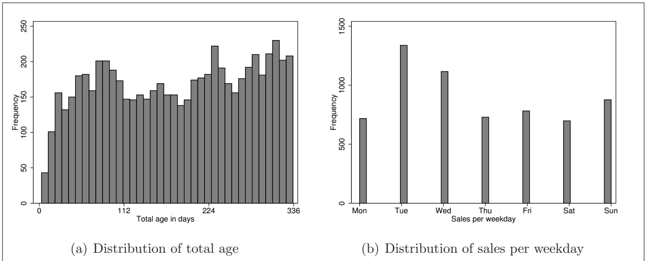
Figure 2: Distributions of Age and Sales
