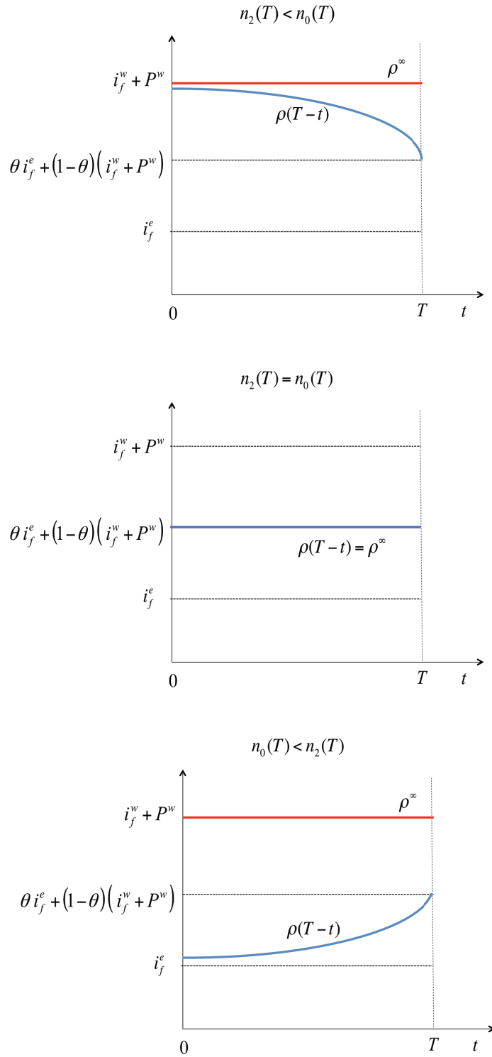
Figure 1: Intraday path of the fed funds rate in an OTC market and in a frictionless market, for different aggregate levels of reserves.
