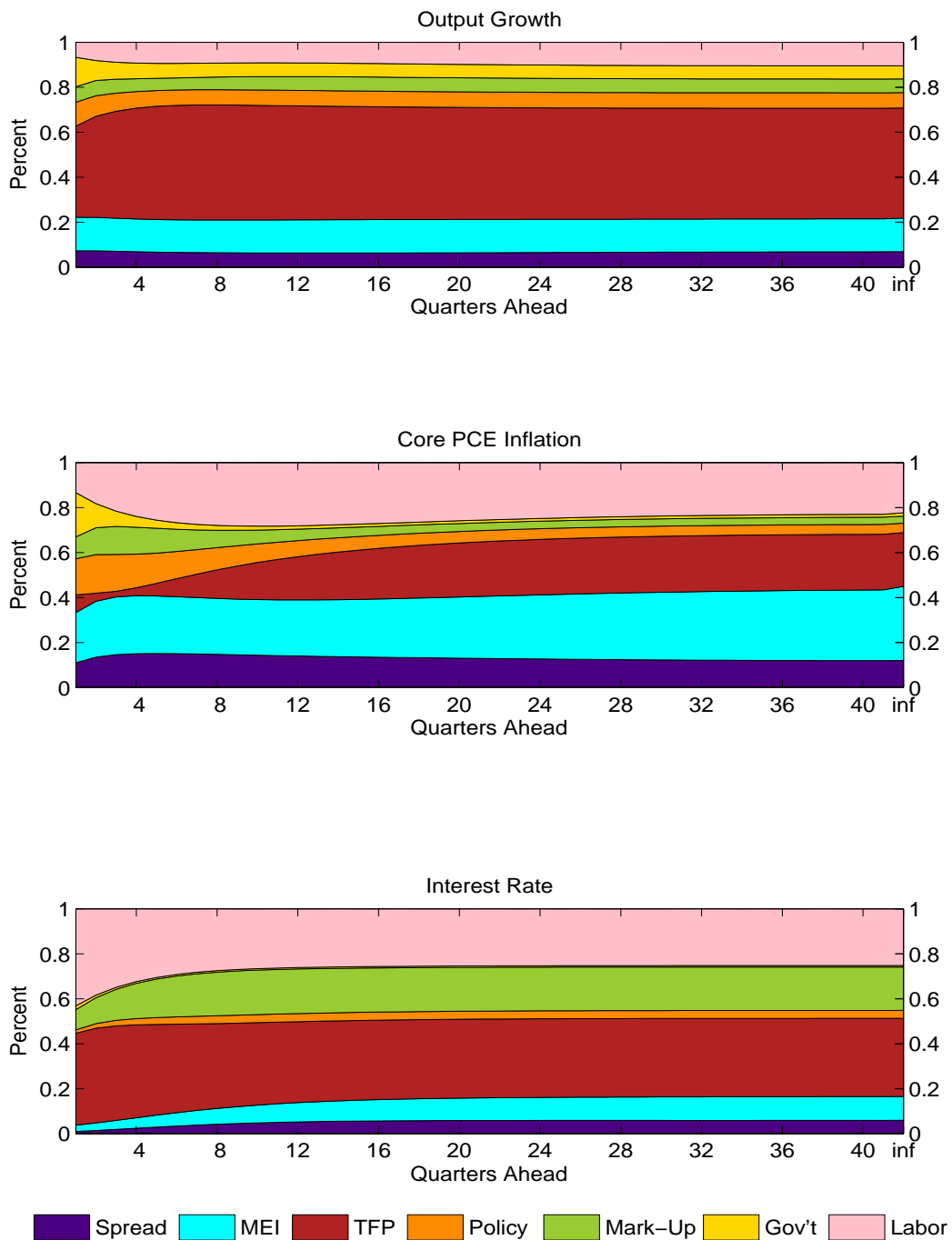
Figure 11: Variance Decomposition
