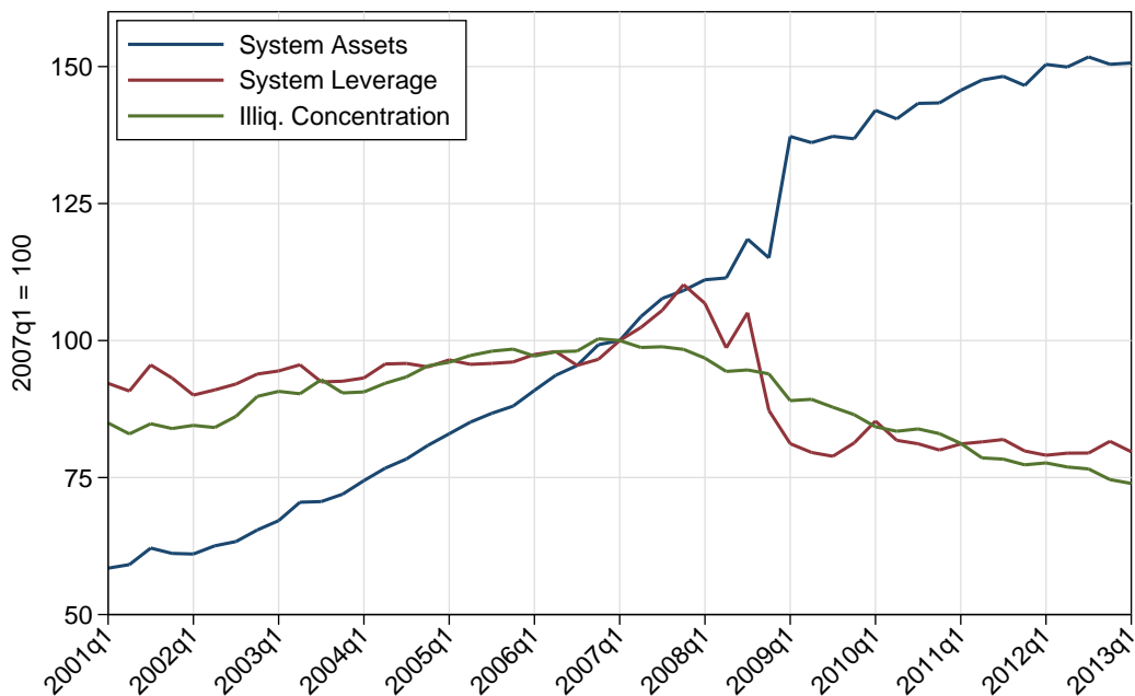
Figure 8: Decomposition of aggregate vulnerability into factors (BHCs).
