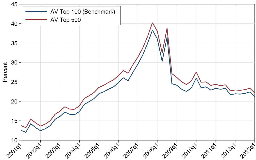
Figure 23: Aggregate vulnerability using the largest 100 banks (benchmark) versus using the largest 500 banks (BHCs).
