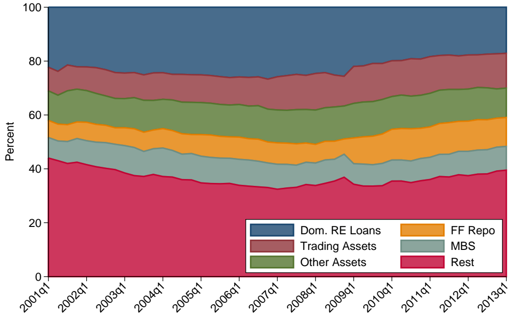
Figure 3: System-wide portfolio shares of asset classes (BHCs).
