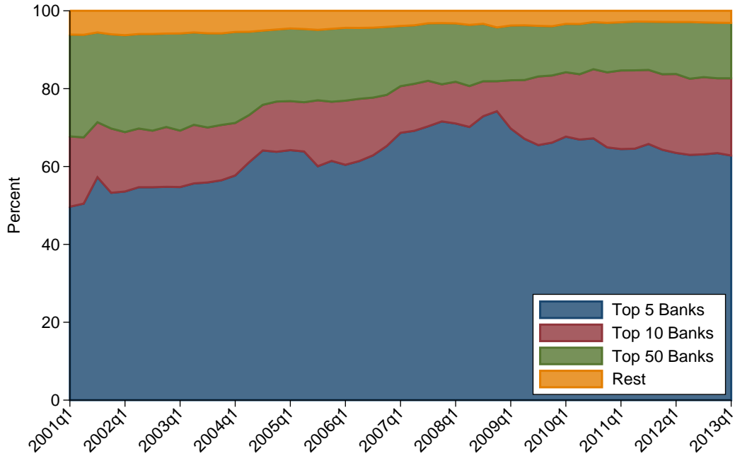
Figure 5: Contribution to aggregate vulnerability by bank size (BHCs).
