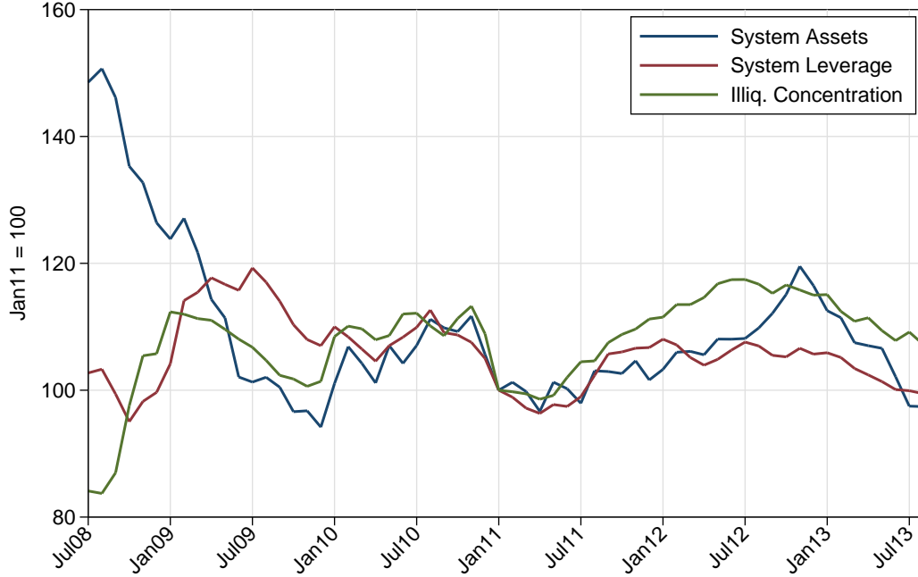
Figure 17: Decomposition of aggregate vulnerability into factors (broker-dealers).
