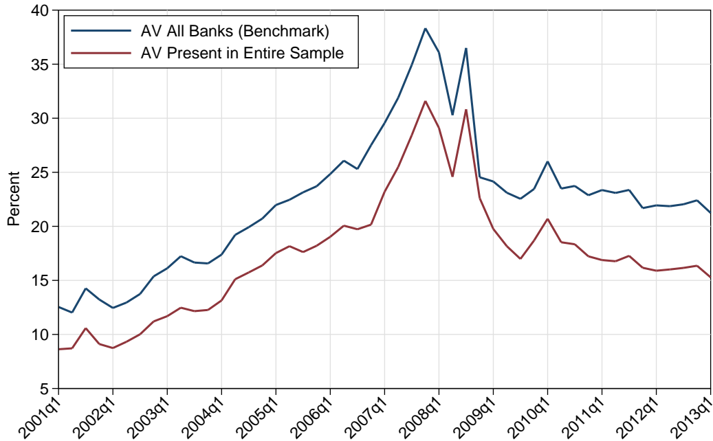
Figure 25: Aggregate vulnerability using the top 100 banks (benchmark) versus using the top 100 banks that have data for every quarter (BHCs).
