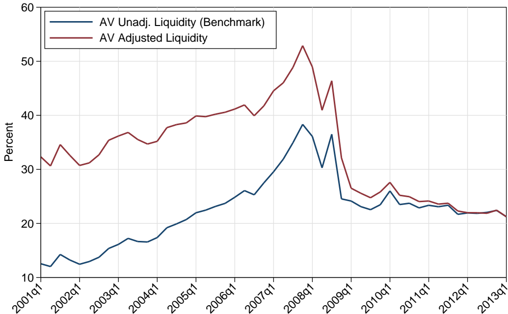
Figure 21: Aggregate vulnerability when liquidity is not time-varying (benchmark) versus liquidity that increases one-for-one with market size (BHCs).
