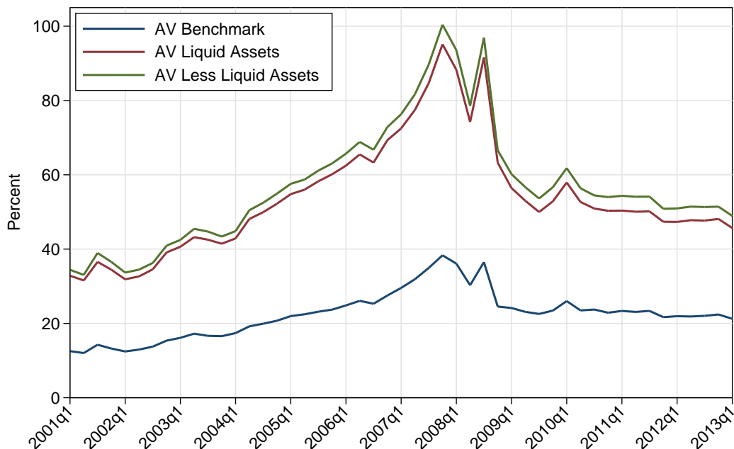
Figure 12: Aggregate vulnerability where every asset is as liquid as equities (benchmark) and with liquidity conditions of Table 2 (BHCs).
