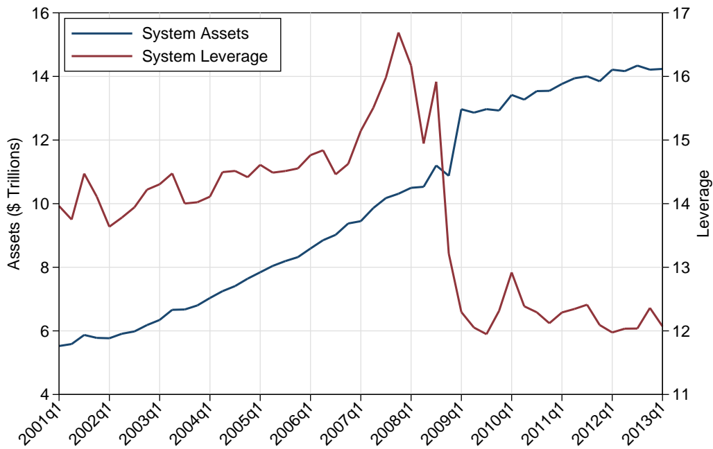
Figure 2: System assets and system leverage for BHCs.
