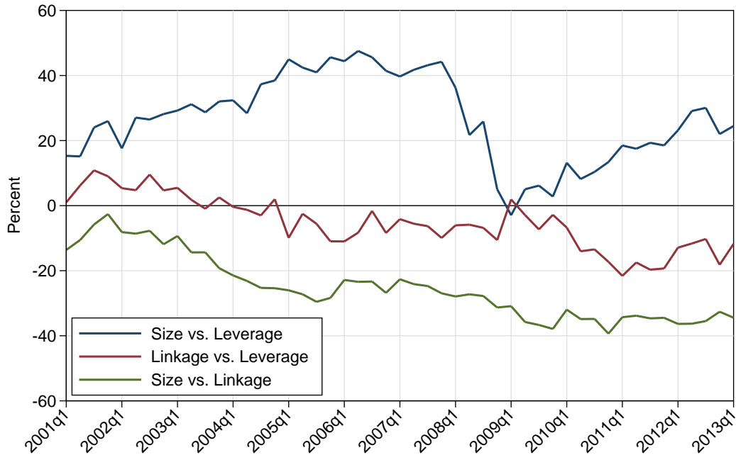
Figure 9: Cross-sectional rank correlations of bank size, leverage and illiquidity linkage (BHCs).
