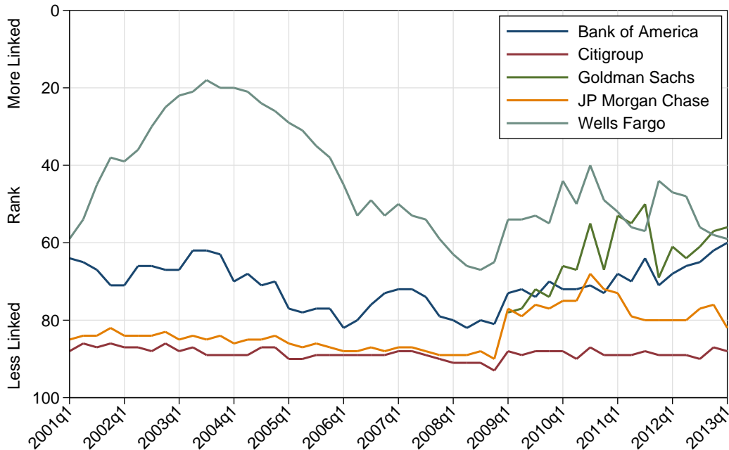
Figure 10: Rank of illiquidity linkage for the most systemic banks (BHCs).
