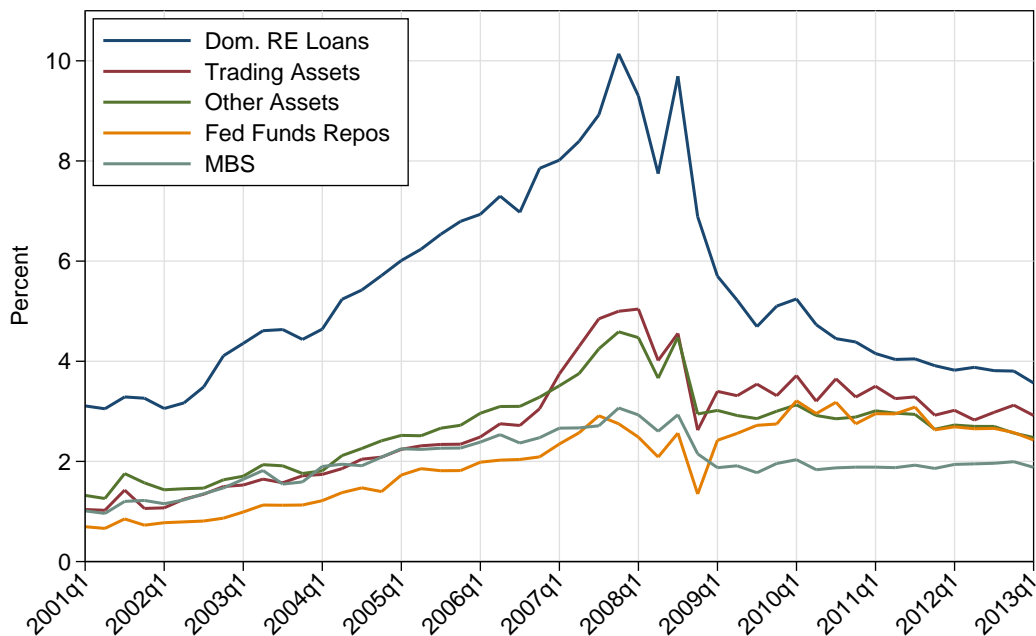
Figure 7: Fire-sale externality of most systemic asset classes (BHCs).
