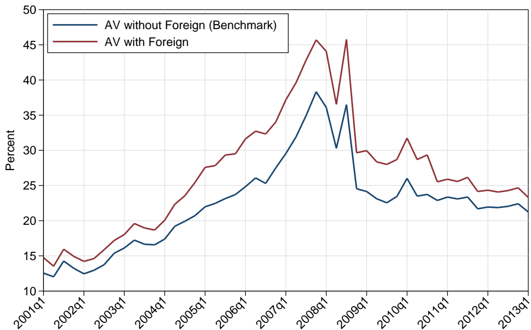
Figure 24: Aggregate vulnerability excluding foreign banks (benchmark) versus including them (BHCs).
