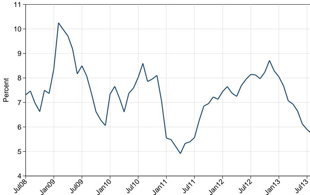
Figure 16: Benchmark aggregate vulnerability for a 0.1 percent shock to all assets with homogeneous asset liquidity (broker-dealers).
