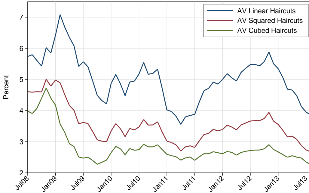
Figure 18: Aggregate vulnerability measures for the heterogeneous liquidity scenarios in Table 4 (broker-dealers).
