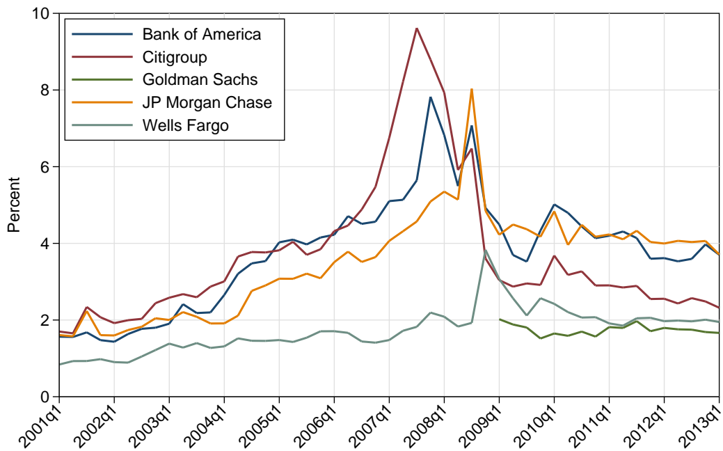
Figure 6: Fire-sale externality of most systemic banks (BHCs).
