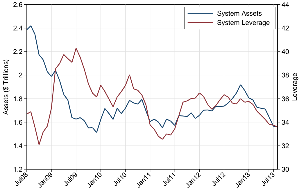
Figure 13: System assets and system leverage for broker-dealers.
