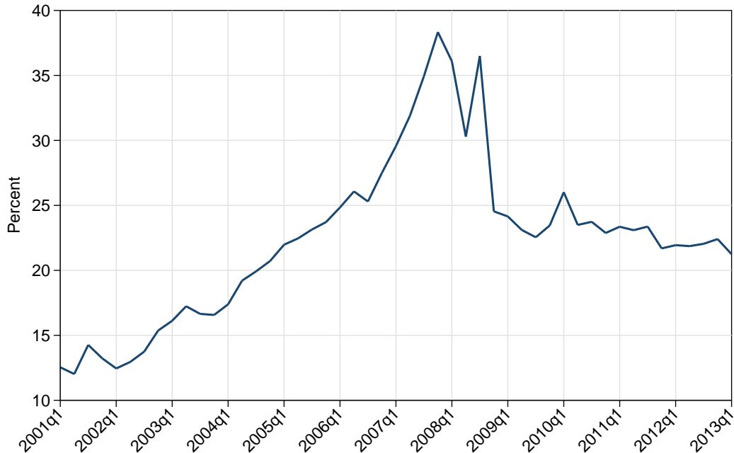
Figure 4: Benchmark aggregate vulnerability, the percentage of system equity capital lost due to fire-sales after the price of all assets go down by 1 percent (BHCs).
