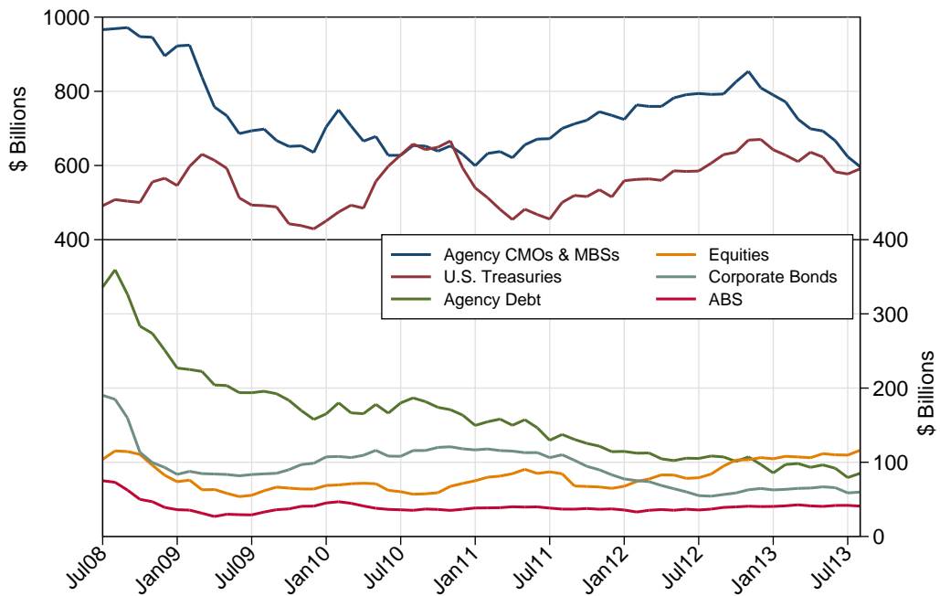
Figure 14: Sizes of main asset classes (broker-dealers).
