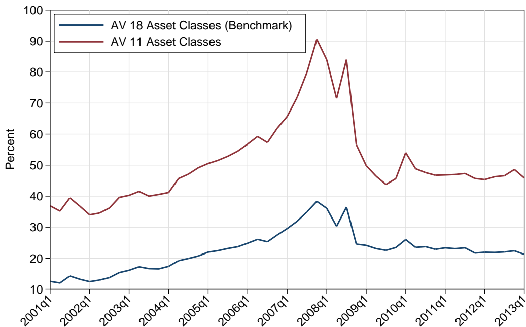
Figure 22: Aggregate vulnerability using eighteen asset classes (benchmark) versus collapsing them to eleven (BHCs).
