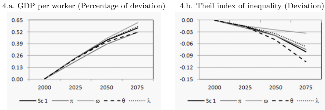
Figure 4. Robustness analysis
