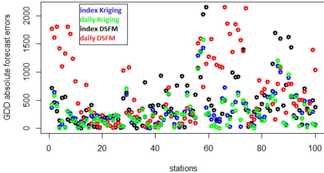
Fig. 8: Absolute forecast errors from Index Kriging, Daily Kriging, Index DSFM, and Daily DSFM for all stations compared to true observations in 2009
