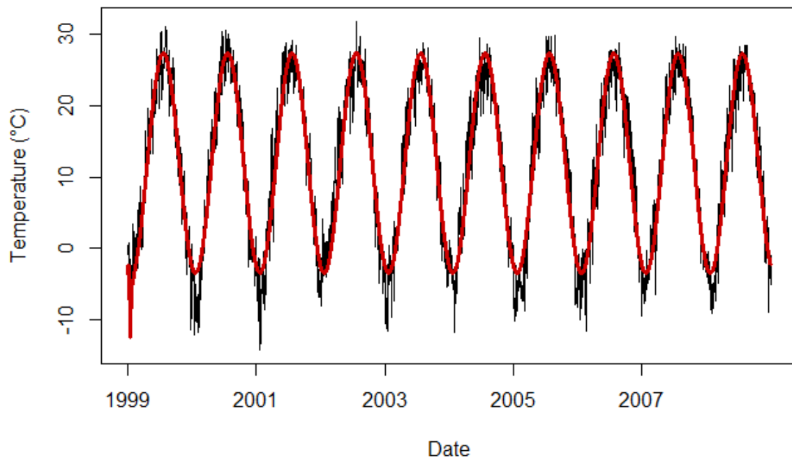
Fig. A2: Ten years of temperature data (black) with the fitted conditional mean function (red) in station Quzhou
