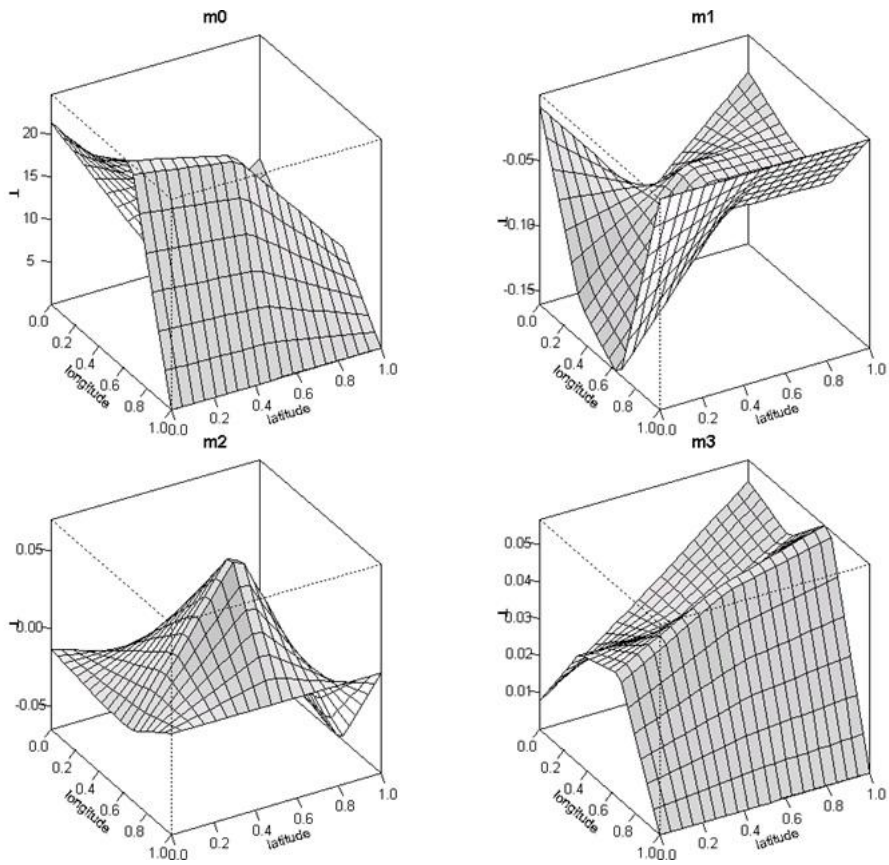
Fig. 5: Estimated factor functions m_0, m_1, m_2, m_3 for the Daily DSFM approach
