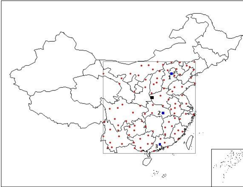
Fig. 2: Map of Chinese weather stations in the study area (The blue squares show the three reference stations: 1=Beijing, 2=Wuhan, and 3=Guangzhou. The black square shows Lushi and is used for illustrating geographic basis risk.)
