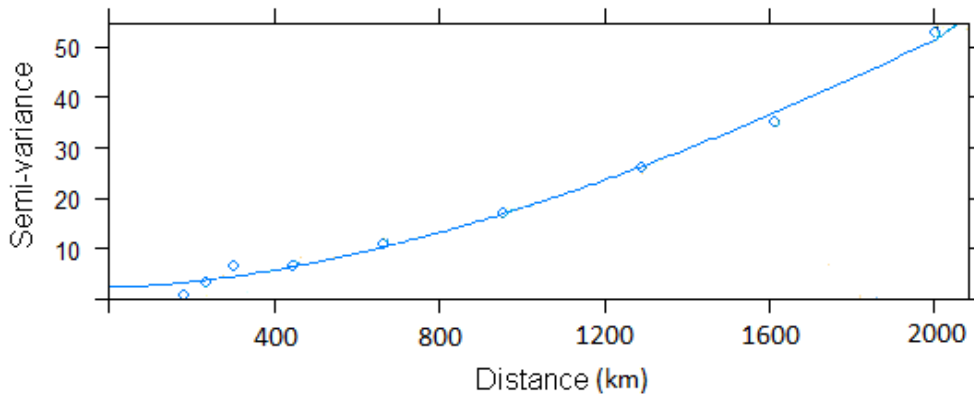
Fig. 3: The experimental (circle) and the theoretical Stein-Matern variogram (line) on January 1 st , 1999
