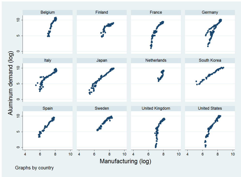
Figure 13: Scatter plot of per capita value added by manufacturing (horizontal axis) and per capita aluminum use (vertical axis).
