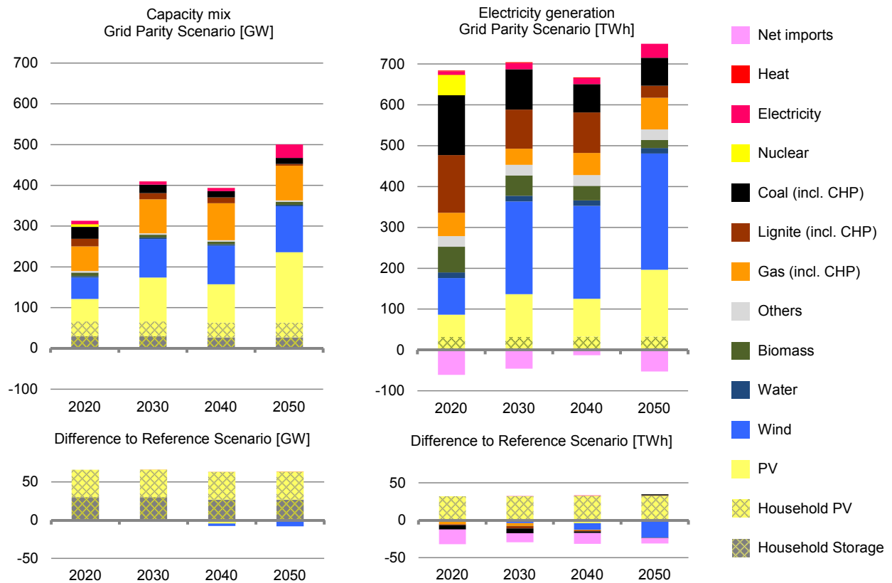
Figure 6: Capacity and generation mix in the ‘Grid Parity Scenario’ and difference to the ‘Reference Scenario’
