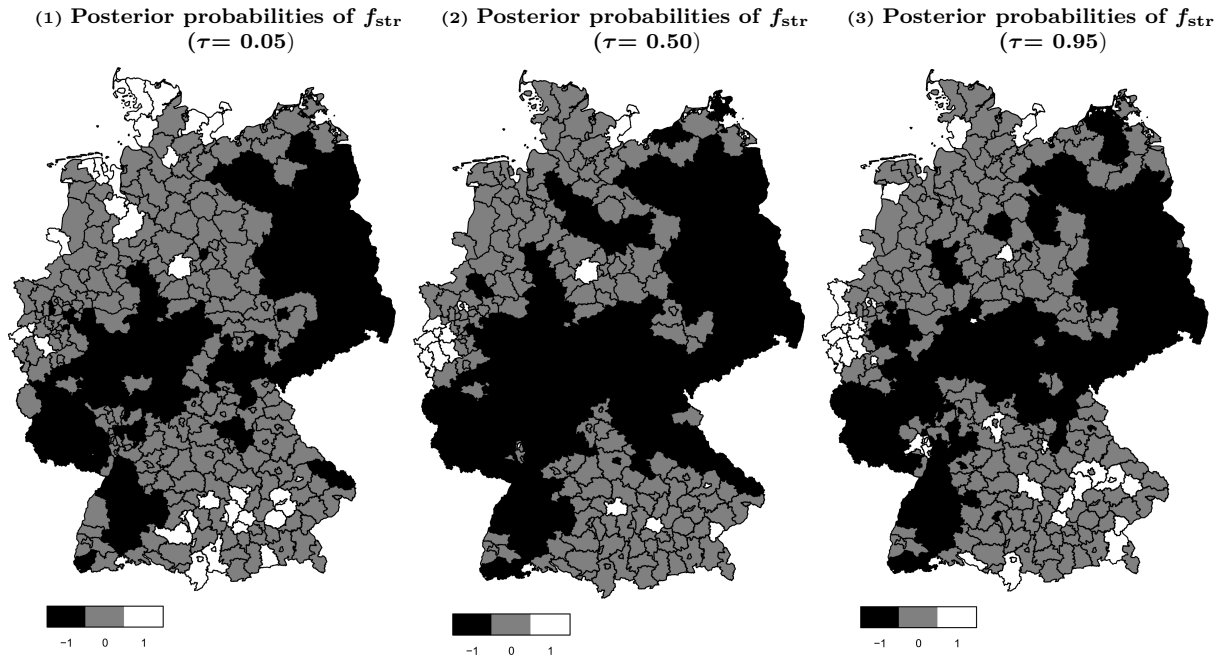
Figure 2. Posterior probabilities of the structured spatial effect f_{str} based on a nominal level of 80%.
