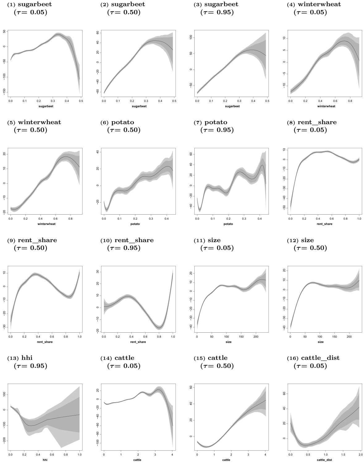
Figure 1. Semi-parametric effects with 80% and 95% pointwise credible intervals.
