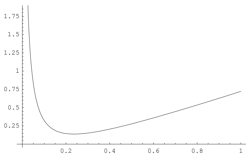
Figure 8 : The f – map with K > 1
