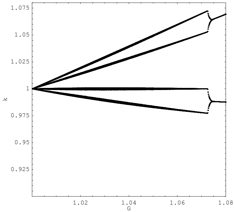
Figure 9 : The Bifurcation Map \sigma = 5 , 1.08 > G > 1
