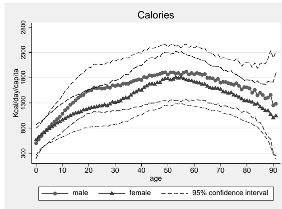
Figure 1: Estimated calories-age curves using non-linear model with roughness penalty \lambda = 100 - weighted average over 1975-2000.
