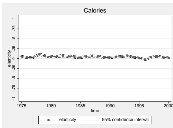
Figure 4: Estimated calories elasticity trend, \lambda = 100 .
