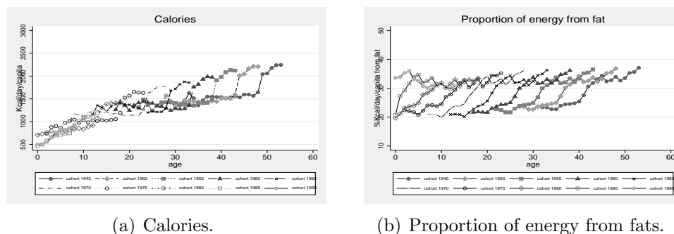
Figure 3: Estimated intakes-cohort curves using non-linear model with roughness penalty \lambda = 100 .
