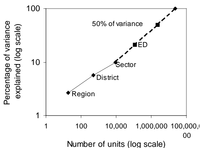
Figure 3 Relationship between area inequalities and number of spatial units analysed
