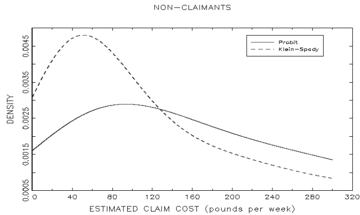
Figure 4 Kernel estimates of the distributions of stigma/claim costs for IS non-recipients (sample 2)
