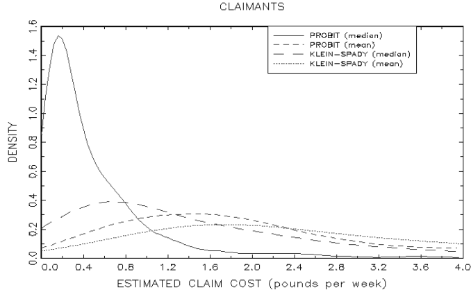
Figure 3 Kernel estimates of the distributions of stigma/claim costs for IS recipients (sample 2)
