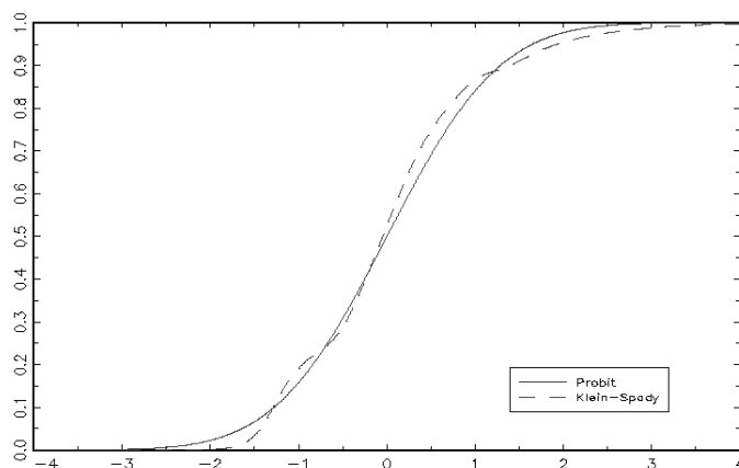
Figure 2 Estimated distribution functions for the probit and Klein-Spady models.
