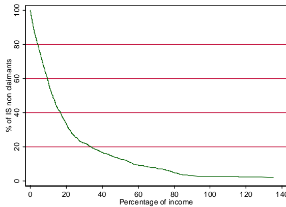
Figure 1 Distribution of IS non-claimants by size of unclaimed benefit as a proportion of original income
