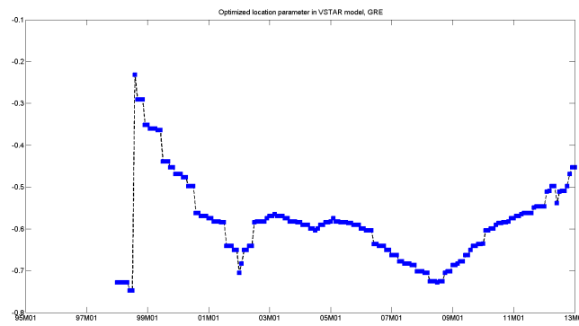
Figure 13: Optimized location parameter VSTAR model, Greece
