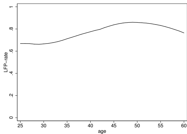
(b) Medium-Skilled
