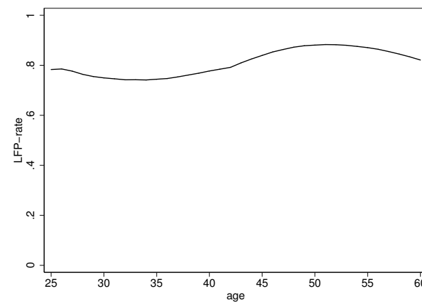
(c) High-Skilled
