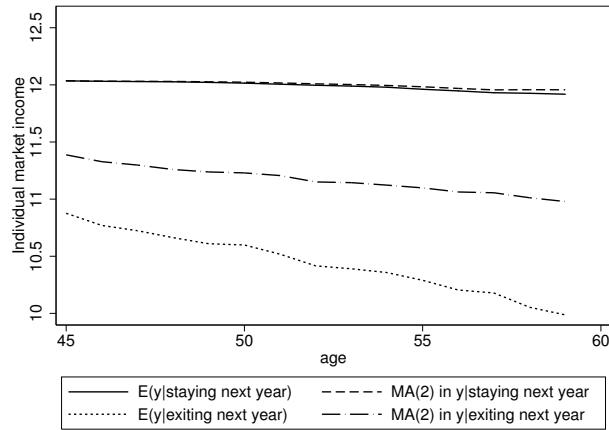
(a) Low-Skilled
