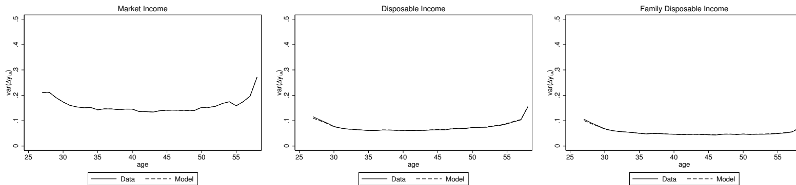
(b) Medium-Skilled
