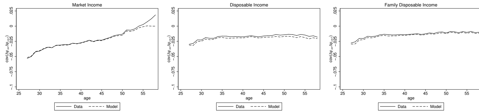
(a) Low-Skilled
