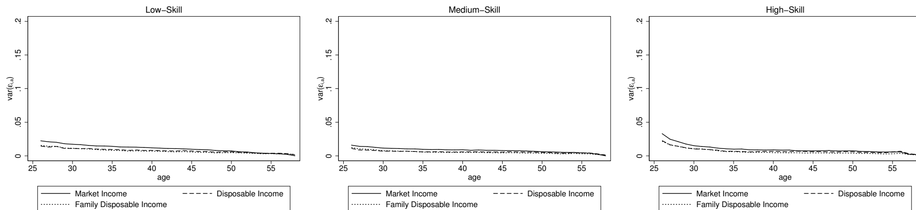
(a) Low-Skilled
