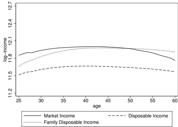
(a) Low-Skilled
