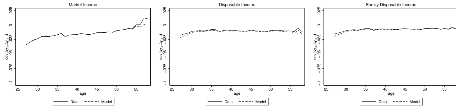
(b) Medium-Skilled
