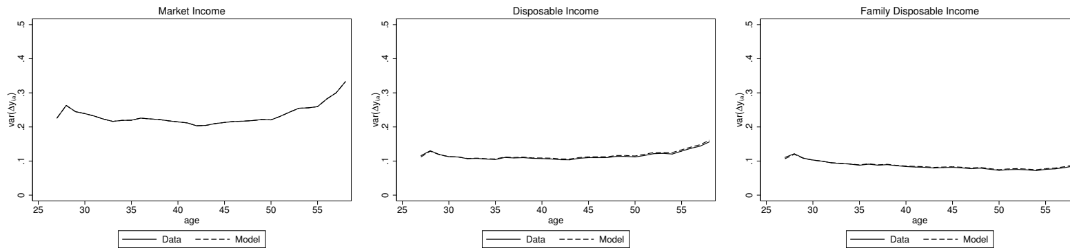
(a) Low-Skilled
