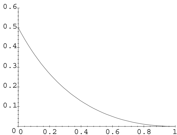
Figure 2: Concentration Parameter \tau , \sigma_\eta^2 = \sigma_v^2 = 1 , T = 3 . Source: Blundell and Bond (1998)
