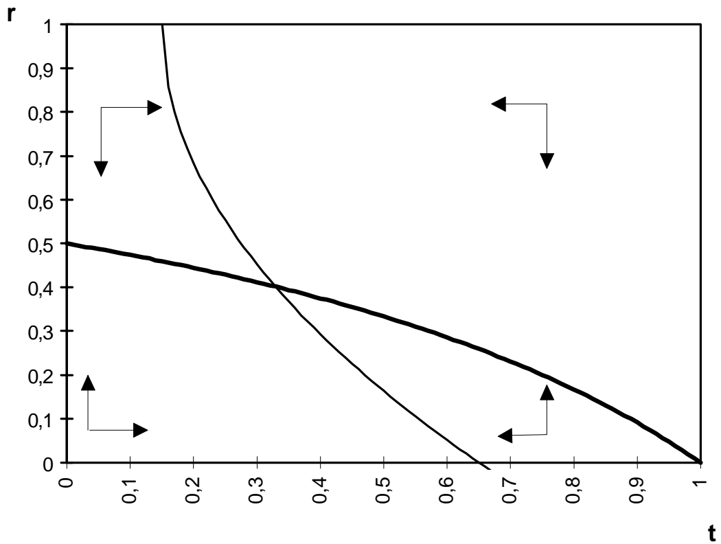
Figure 3: Graphs of g(t) (thickly drawn) and f(t; a) when there is only one intersection, a = 0.5 .
