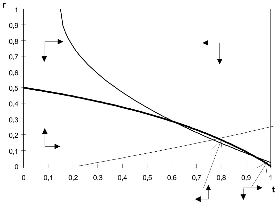
Figure 4: Graphs of g(t) (thickly drawn) and f(t; \mathbf{a}) when there are two intersections, \mathbf{a} = 0.89 . The thinly drawn, increasing curve is the graph of h(r; \mathbf{a}) , indicating the types of the stationary points.
