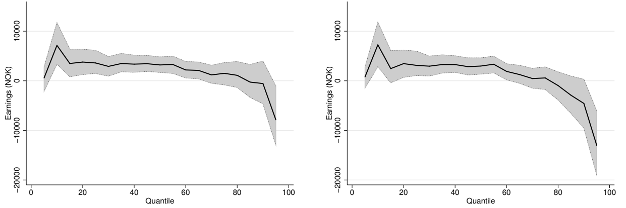
(a) CIC-estimates
