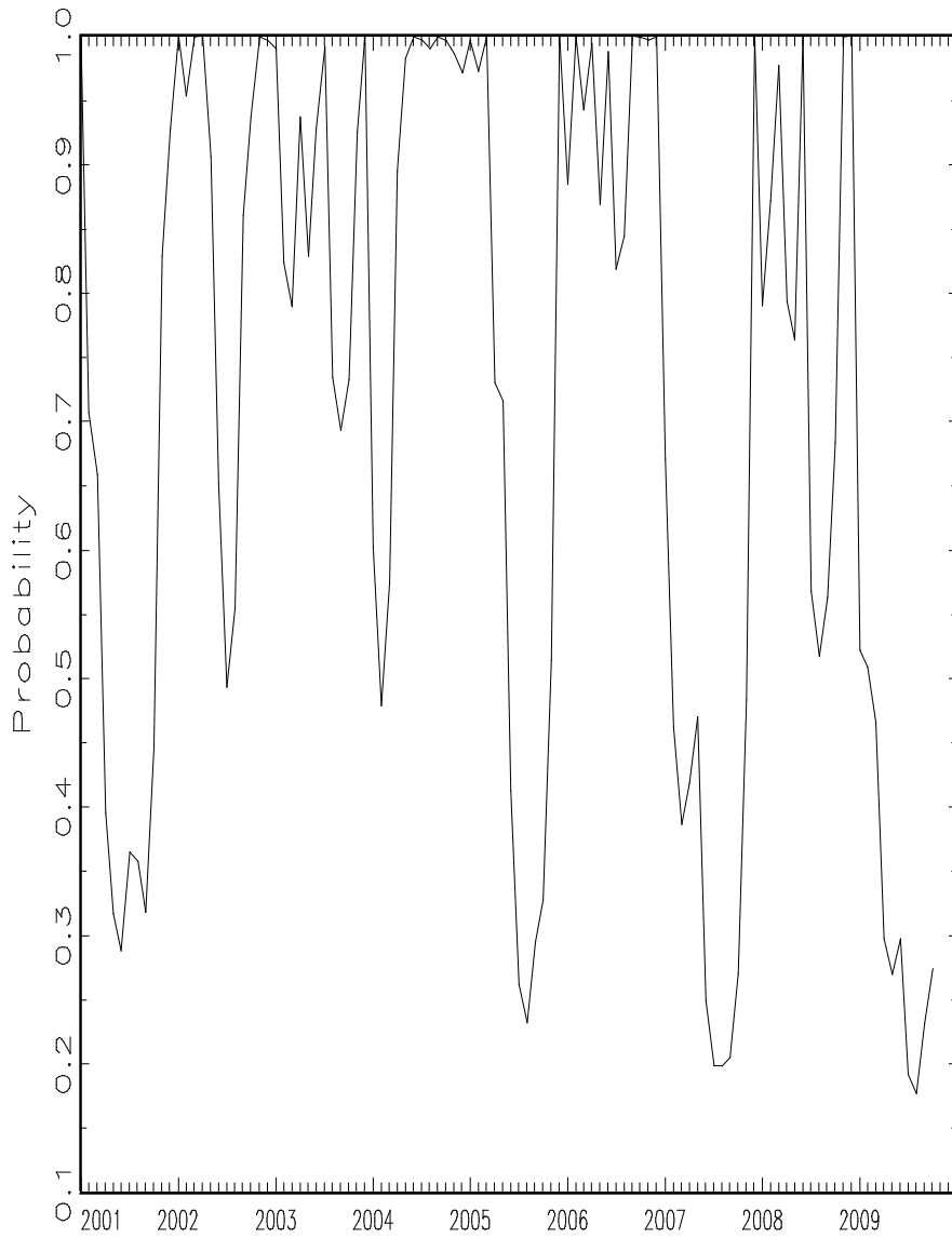
Figure 2: Smoothed probability in regime 2 (high and volatile inflation)
