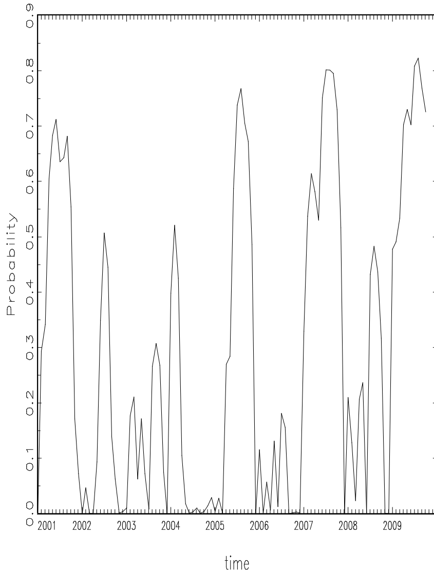
Figure 1: Smoothed probability in regime 1 (low and stable inflation)
