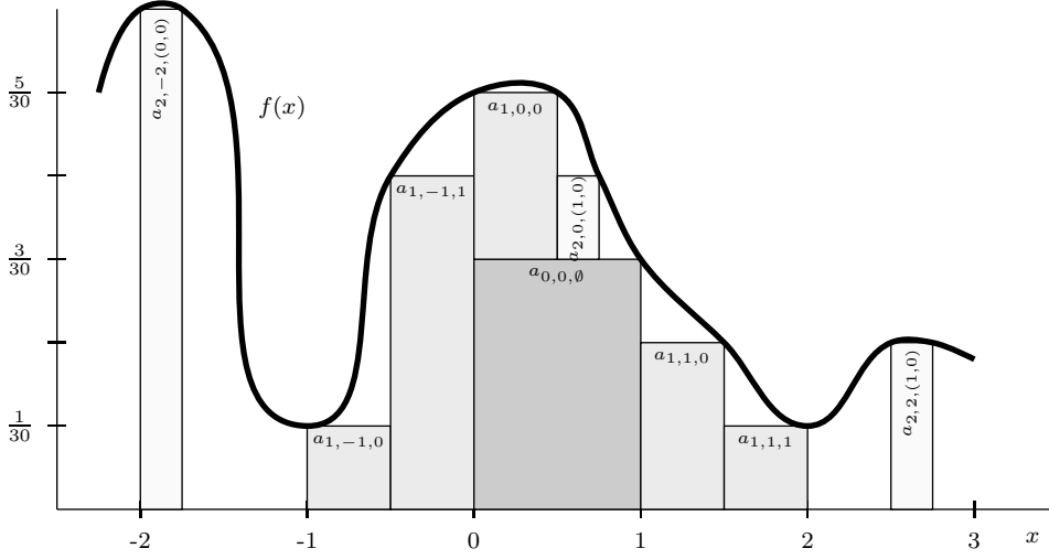
Figure 1: Approximation of a continuous spectral function f by the step function f_2 defined in (3). The corresponding coefficients are given in Example 1. Note that the bars a_{nki} do not necessarily touch the graph of f .
