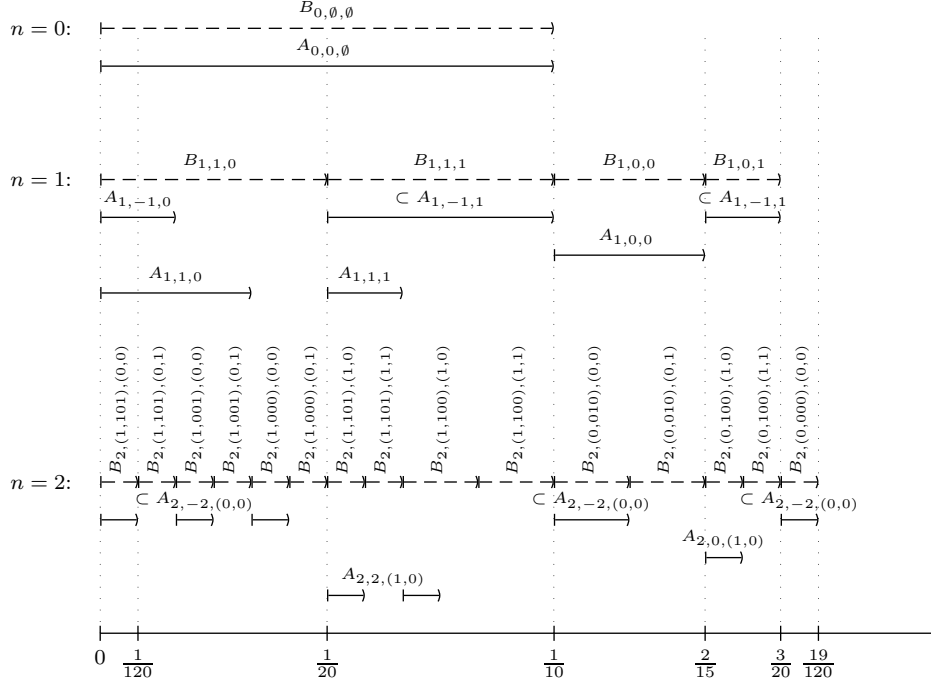
Figure 2: Jointly successive construction of B_{nbi} and A_{nki} (top to bottom) using (16) and (35) up to n = 2 . The corresponding coefficients are given in Example 1. In the figure by “ \subset X ” we denote a subset of a set X .
