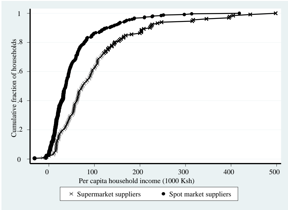
Figure 4. Cumulative distribution of annual per capita household income by market channel Note: The Kolmogorow-Smirnov test statistic of 0.361 indicates that the two distributions are statistically different ( p=0.000 ).
