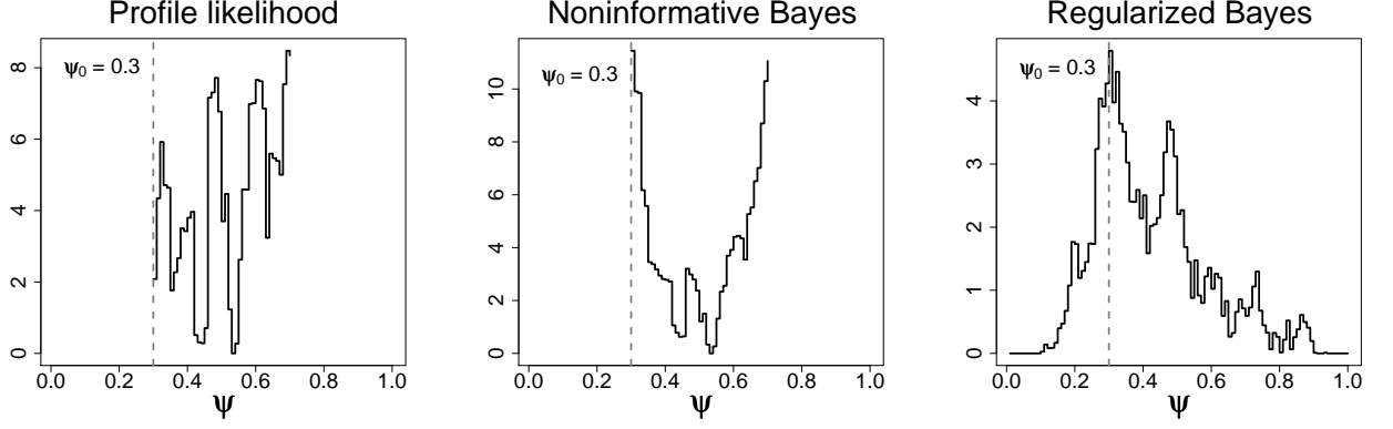
Figure 1: For a sample run corresponding to setting 1C of Section 6, \ell_p(\psi) is shown on the left, \log p_{nB}(\psi|\mathbf{y}, \mathbf{X}, \mathbf{q}) in the middle and \log p_{rB}(\psi|\mathbf{y}, \mathbf{X}, \mathbf{q}) on the right.
