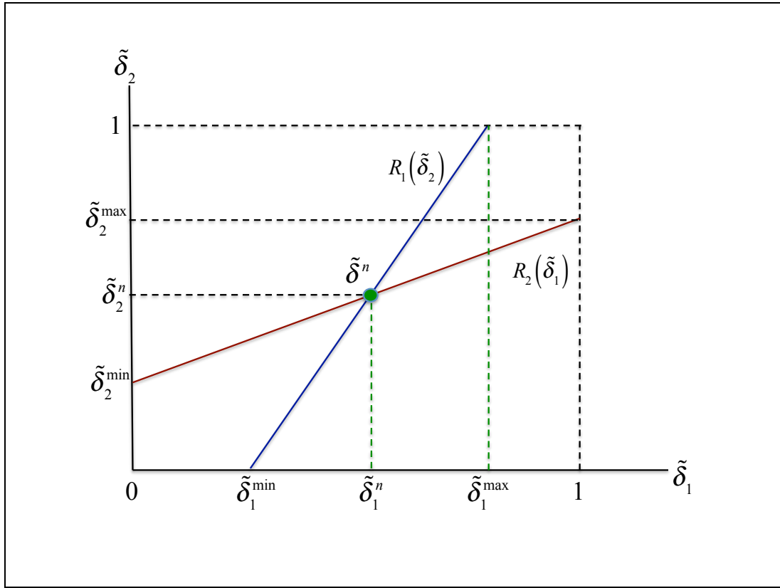
Figure 2: Two-Workers – Nash Equilibrium Reservation Sickness
