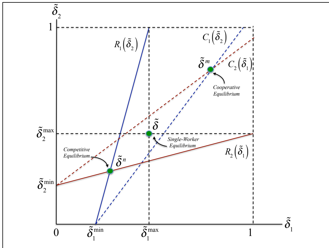
Figure 5: Cooperative and Nash Solutions (i)
