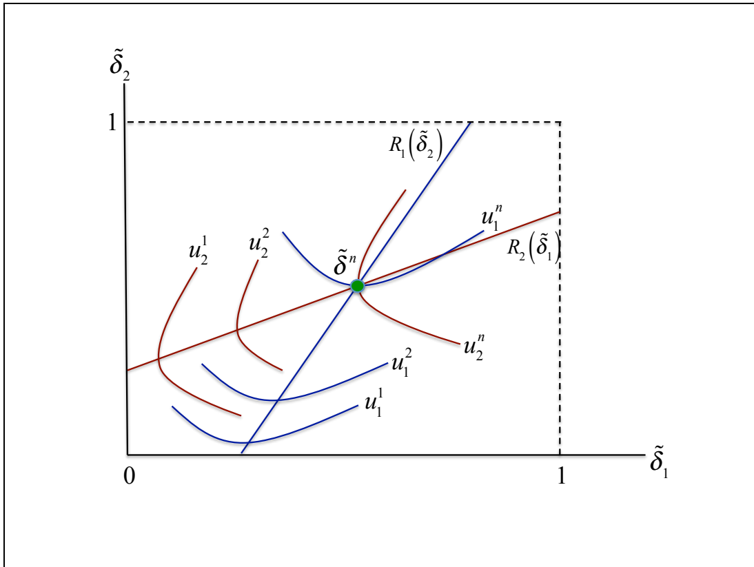
Figure 3: Pareto Inefficiency of Nash Equilibrium
