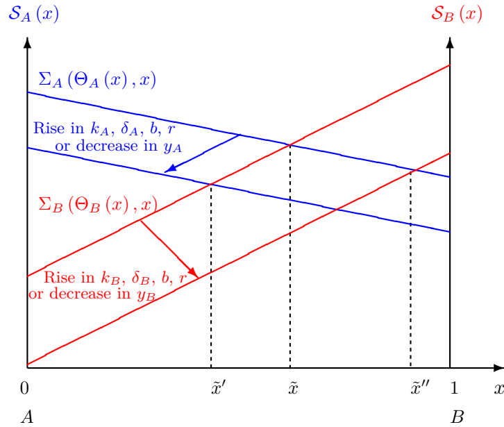
Fig. 3. Comparative statics
