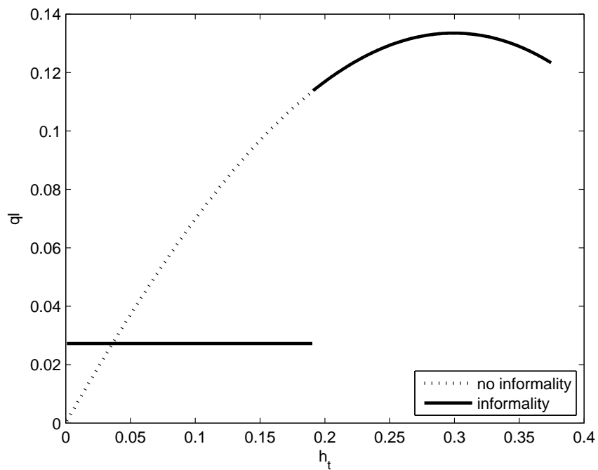
(b) q_l(h_t)
