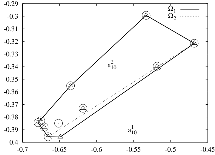
Figure 2: Solid angle in year 1 and 2.
