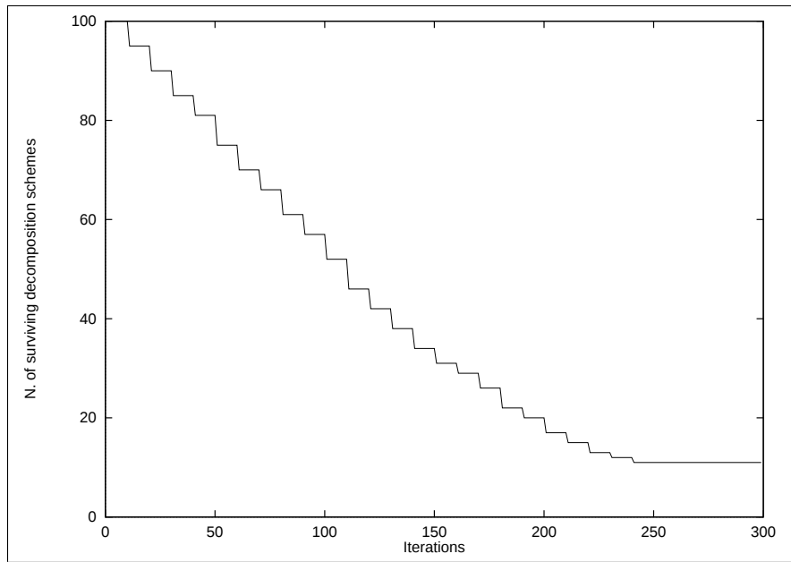
Figure 5: Diversity of surviving decomposition schemes.
