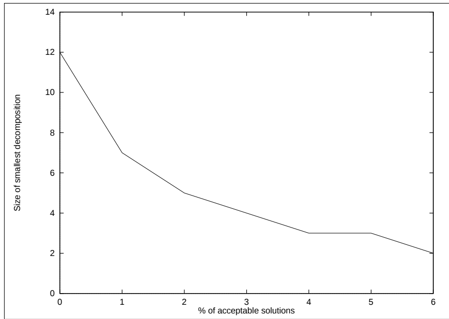
Figure 2: Near decomposability.
