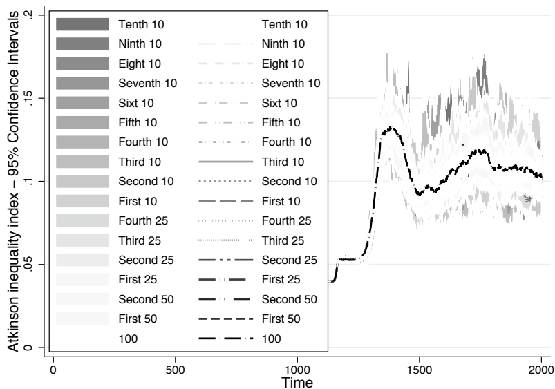
Figure 6: Atkinson inequality index: averages and confidence intervals . The figure shows the confidence areas of the different averages (over samples of 100, 50, 25, and 10 replicates) superimposed one over the other, starting from 10 replicates' averages. The grey scale goes from dark grey for 10 replicates' averages to white for the 100 replicates average. The figure then shows that very small sections of the 10 replicates' confidence area exceed the 100 runs confidence area, amounting to a very small difference between the confidence areas of the different averages.
