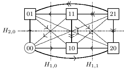
Figure 8: In the 3d social rule a domination path that is a cycle.
