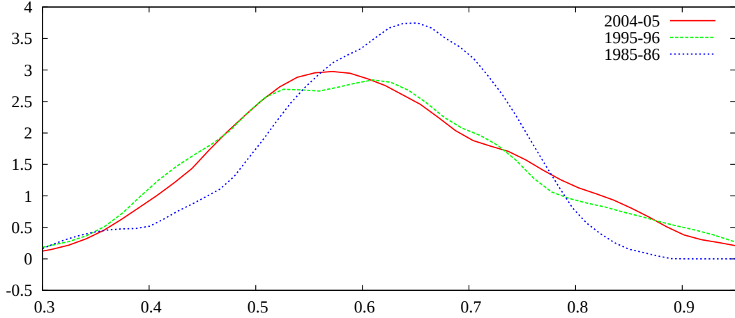
Figure 6: Probability densities of the sectoral concentration index D_{20}^4 in terms of total sales, different years (kernel estimates). The support of these densities is [0.3 \ 0.95] . World's largest firms Osiris (2005) database.
