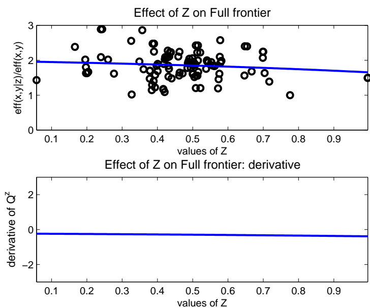
Figure 4: Aggressive Growth US Mutual Funds . Scatterplot and smoothed nonparametric regression of the ratios Q^z = \hat{\lambda}_n(x, y|z)/\hat{\lambda}_n(x, y) on z (top panel) and the estimate of the derivative of Q^z with respect to z (bottom panel).
