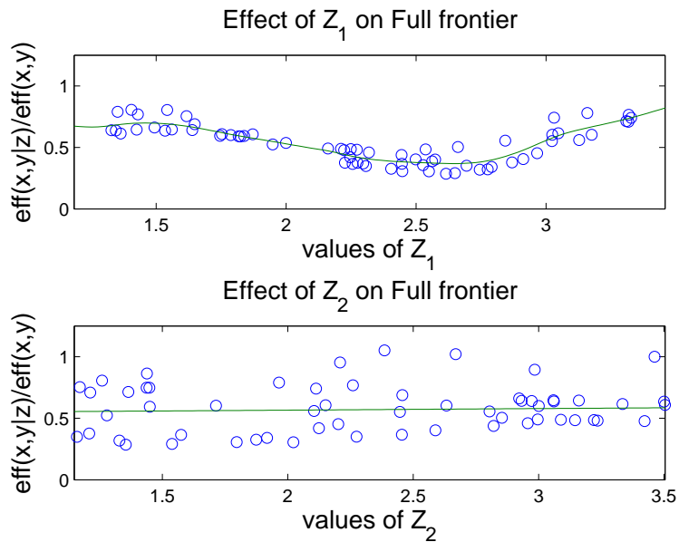
Figure 3: Simulated example with multivariate Z . Marginal views of the surface regression of \hat{\lambda}_n(x,y|z)/\hat{\lambda}_n(x,y) on z at the observed points (X_i, Y_i, Z_i) , viewed as a function of Z_1 (top panel) and as a function of Z_2 (bottom panel).
