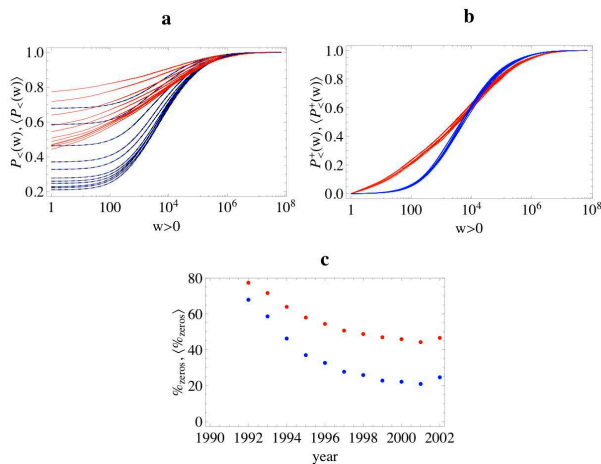
FIG. 16: Edge weights in the weighted directed ITN (red: real network, blue: expectation for the maximum-entropy ensemble with specified out-strengths and in-strengths). a) cumulative distributions of edge weights in the years 1992 (top curves) to 2002 (bottom curves). b) same as the previous panel, but excluding zero weights (missing links). c) percentage of missing links as a function of time.
