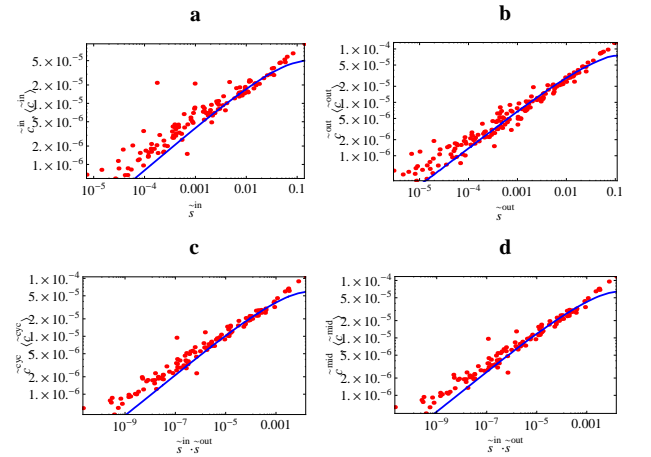
FIG. 11: Weighted clustering coefficients versus vertex strengths in the 2002 snapshot of the real weighted directed ITN (red points), and corresponding averages over the maximum-entropy ensemble with specified out-strengths and in-strengths (blue curves). a) \tilde{c}_i^{in} versus \tilde{s}_i^{in} ; b) \tilde{c}_i^{out} versus \tilde{s}_i^{out} ; c) \tilde{c}_i^{cyc} versus \tilde{s}_i^{in} \cdot \tilde{s}_i^{out} ; d) \tilde{c}_i^{mid} versus \tilde{s}_i^{in} \cdot \tilde{s}_i^{out} .
