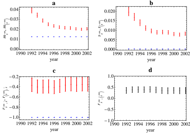
FIG. 3: Temporal evolution of the properties of the (rescaled) average nearest neighbor strength \tilde{s}_i^{nn} in the 1992-2002 snapshots of the real weighted undirected ITN and of the corresponding maximum-entropy ensembles with specified strengths. a) average of \tilde{s}_i^{nn} across all vertices (red: real, blue: randomized). b) standard deviation of \tilde{s}_i^{nn} across all vertices (red: real, blue: randomized). c) correlation coefficient between \tilde{s}_i^{nn} and \tilde{s}_i (red: real, blue: randomized). d) correlation coefficient between \tilde{s}_i^{nn} and \langle \tilde{s}_i^{nn} \rangle . The 95% confidence intervals of all quantities are represented as vertical bars.
