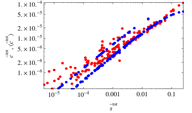
FIG. 10: Total weighted clustering coefficient \tilde{c}_i^{tot} versus total strength \tilde{s}_i^{tot} in the 2002 snapshot of the real weighted directed ITN (red points), and corresponding average over the maximum-entropy ensemble with specified out-strengths and in-strengths (blue curve).
