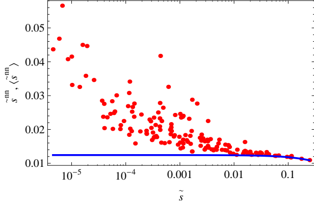
FIG. 1: Average nearest neighbor strength \tilde{s}_i^{nn} versus strength \tilde{s}_i in the 2002 snapshot of the real weighted undirected ITN (red points), and corresponding average over the maximum-entropy ensemble with specified strengths (blue curve).
