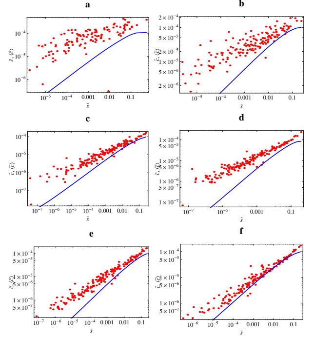
FIG. 7: Weighted clustering coefficient \bar{c}_i versus strength \bar{s}_i in the 2002 snapshots of the commodity-specific (disaggregated) versions of the real weighted undirected ITN (red points), and corresponding average over the maximum-entropy ensemble with specified strengths (blue curve). a) commodity 93; b) commodity 09; c) commodity 39; d) commodity 90; e) commodity 84; f) aggregation of the top 14 commodities (see Ref. [1] for details). From a) to f), the intensity of trade and level of aggregation increases.
