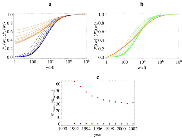
FIG. 5: Edge weights in the weighted undirected ITN. a) cumulative distributions of edge weights in the years 1992 (top curves) to 2002 (bottom curves). Orange: real network; blue: expectation for the maximum-entropy ensemble with specified strengths. b) same as the previous panel, but excluding zero weights (missing links). Orange: real network; green: randomization. c) percentage of missing links as a function of time. Red: real network; blue: randomization.
