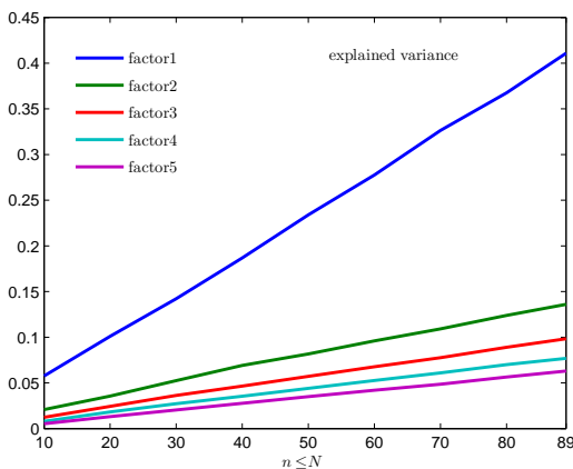
4.1: Explained variance.
